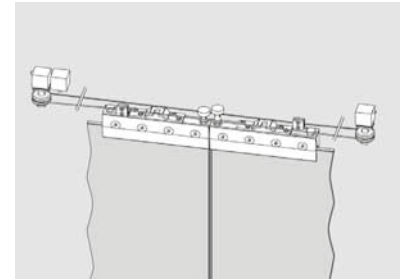
MIC-426-00-021 RS 120 ahşap kanat senkronize set
