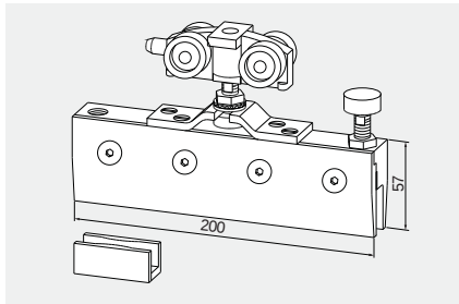
MIC-426-00-001 RS 120 makara seti
